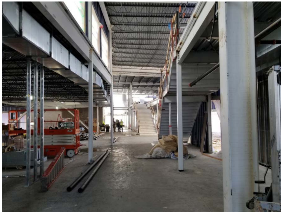
Grand Hall Main Entrance – South Facing View; framing in progress
