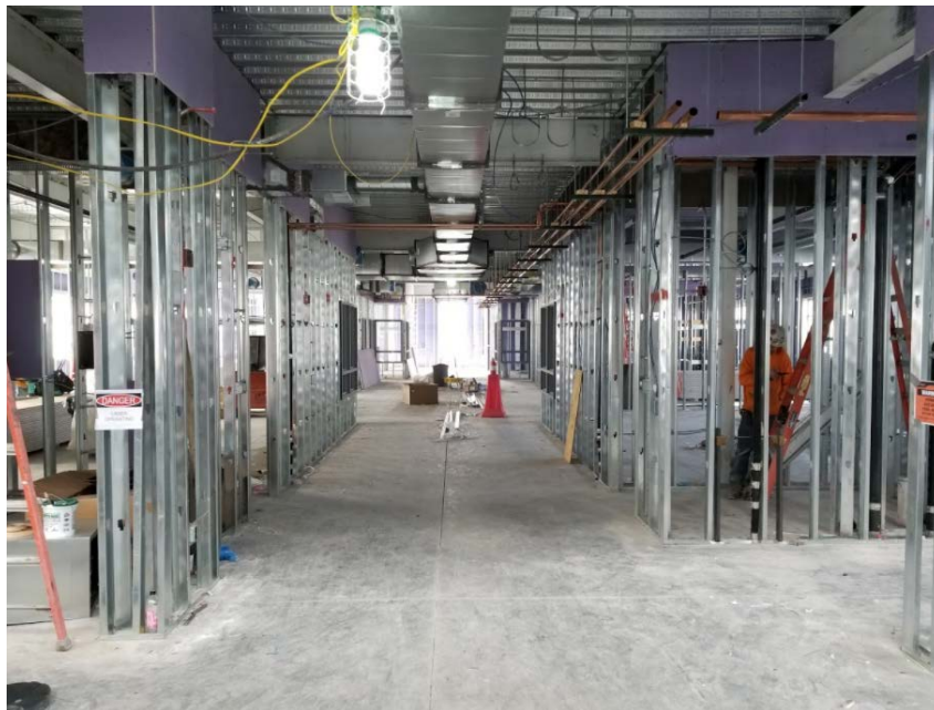
North Classroom Wing (lower level) – West Facing View; plumbing, framing and electrical install in progress
