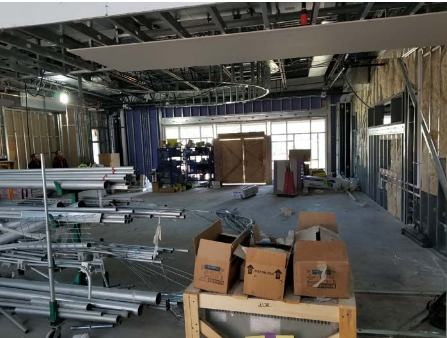
Learning Commons – Insulation and drywall install continues.
